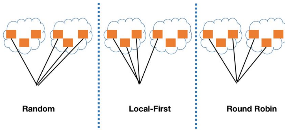
Fig 4: Three traditional scheduling Graph
