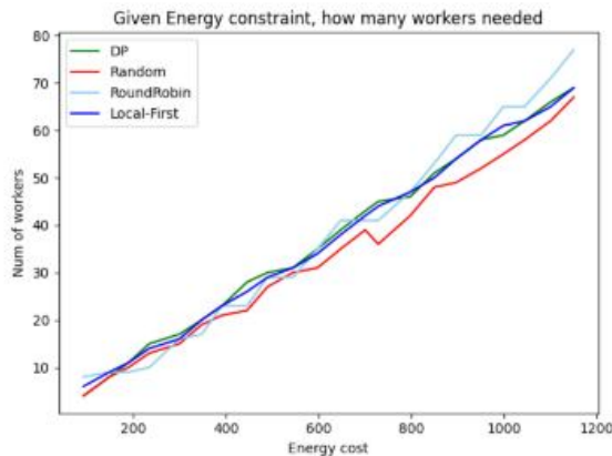
Figure 7: With similar Energy constraint, how many workers needed
