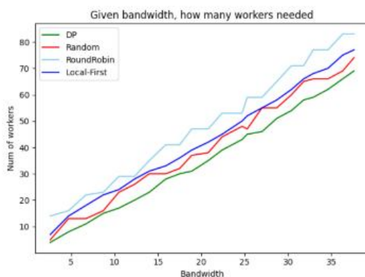
Fig 5: With similar bandwidth, how many workers needed
