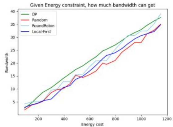
Figure 8: With similar Energy constraint, how much bandwidth can get
