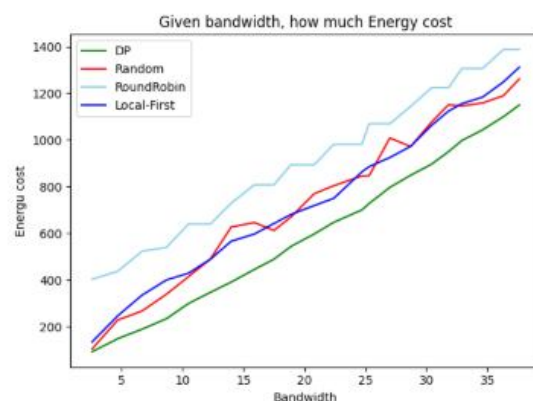
Fig 6: With similar bandwidth, how much Energy cost
