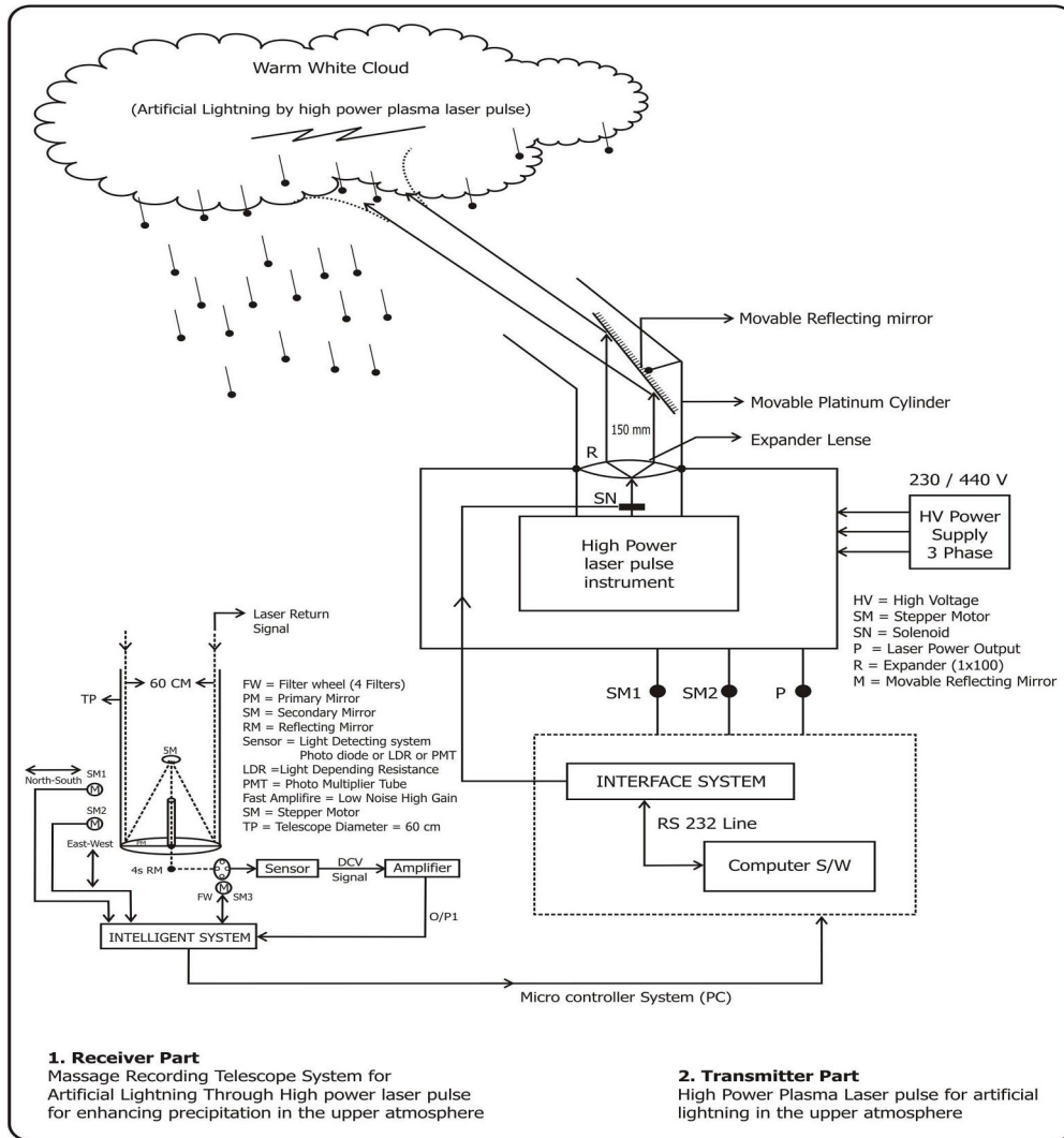
Figure 2 :: Experiment Setup
