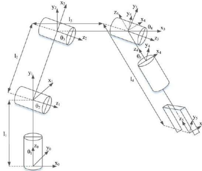
Figure 3 Kinematic scheme of the 5DOF robotic arm
