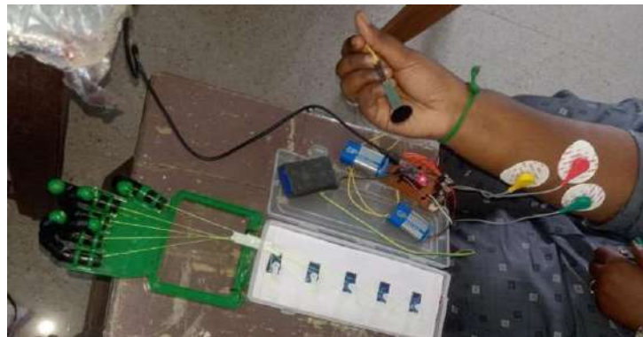
Figure 4 Output Setup
