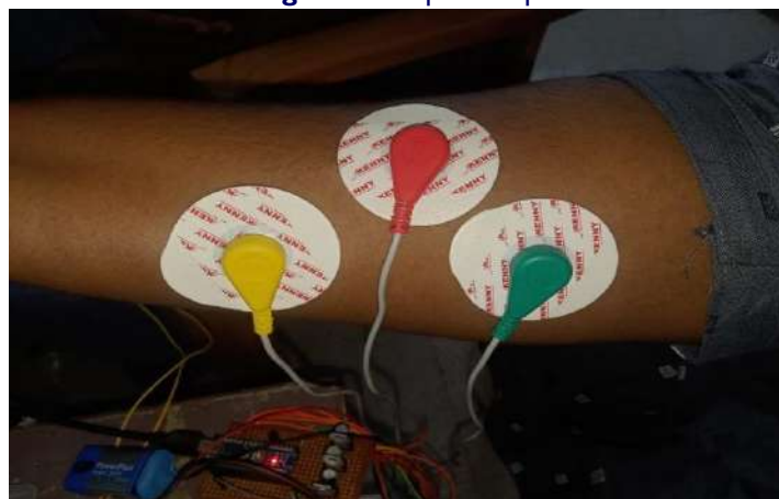
Figure 5 EMG electrodes
